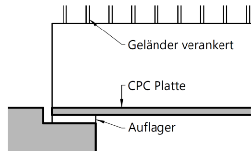
Widerlager
